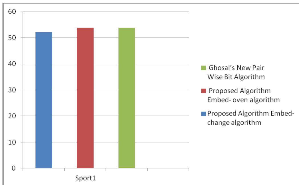
Figure (5-37) shows the PSNR test for Sport1 image
